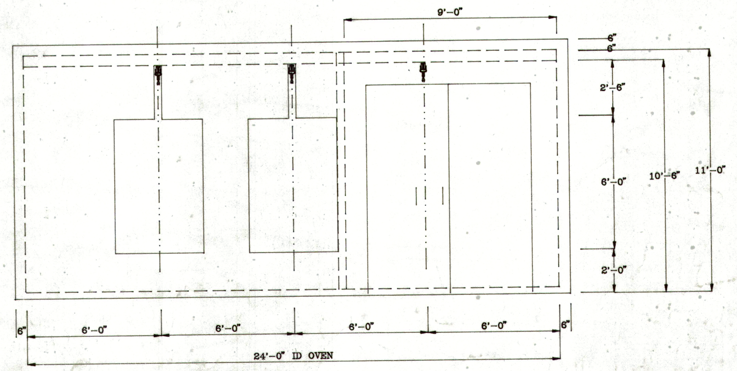
END VIEW/BAKE OVEN SCALE: 3/8"
