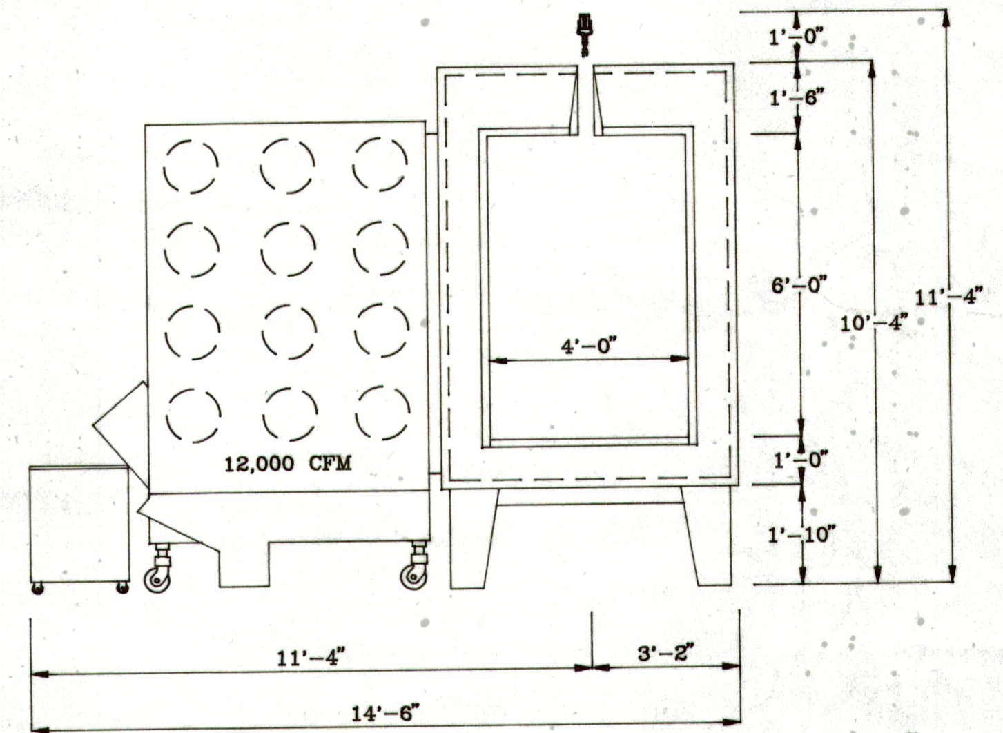
END VIEW/POWDER BOOTH SCALE: 3/8"
