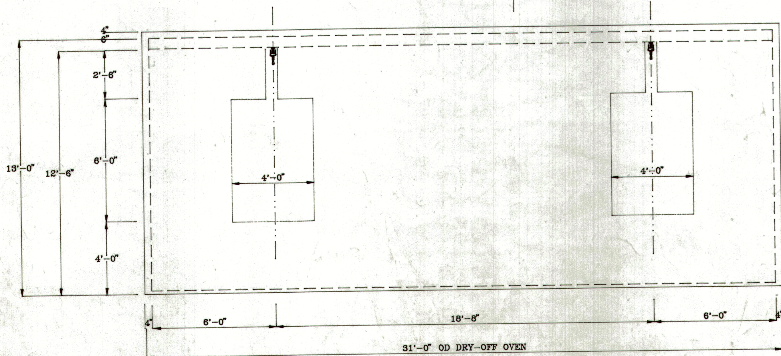
END VIEW/DRY-OFF OVEN SCALE: 3/8"
